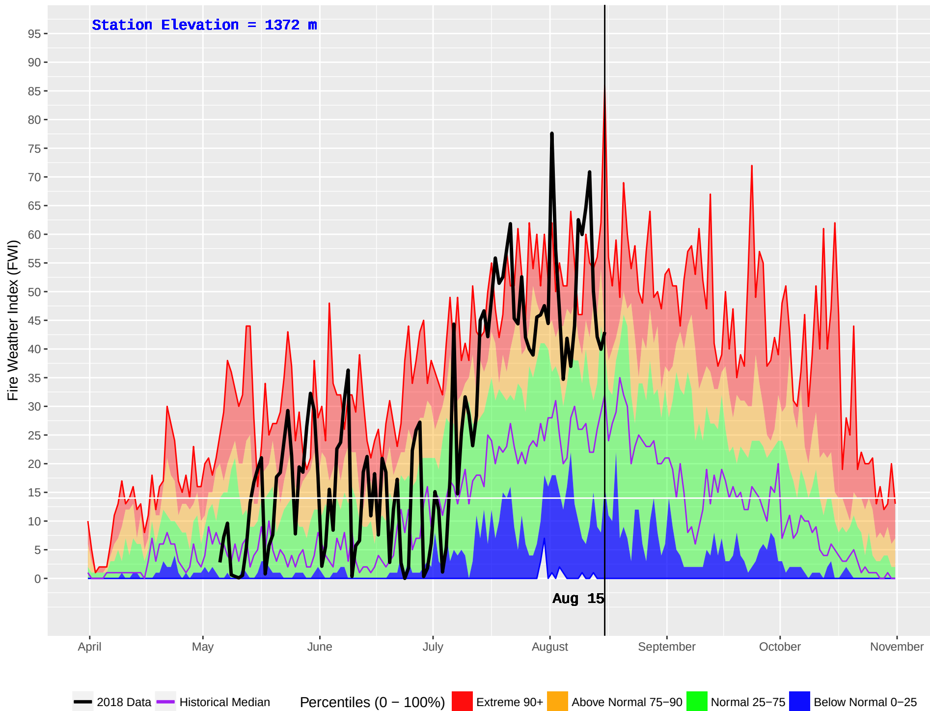
CHERRY LAKE (791) : Historical (1989–2016) and Current (2018) Daily Fire Weather Index (FWI)
